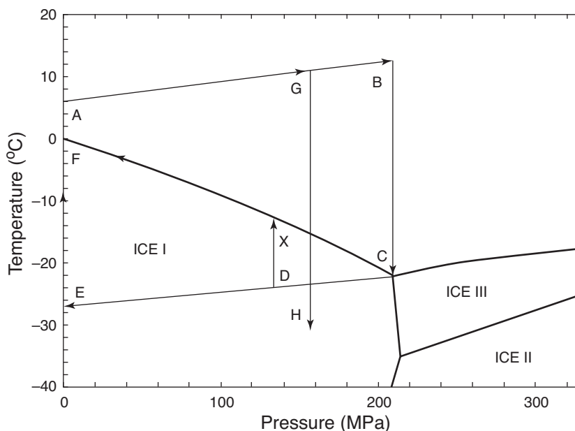
Figure 12.6 Phase diagram of water, with pathways followed during HPSF and PAF freezing processes. ABCF: rapid release HPSF; ABCDXF: slow release HPSF; AGH: PAF. (From Norton et al. (2009).)
