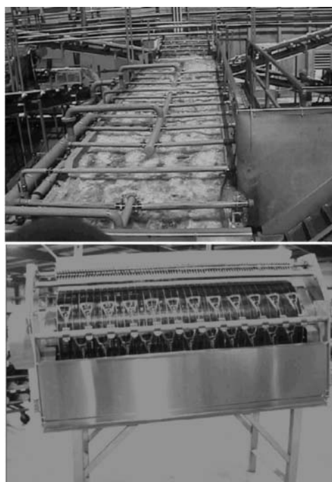
Figure 30.6 Green beans washing line (top) and stem snipper (bottom). (Courtesy: Lyco Manufacturing, Inc., Columbus, Wisconsin, USA.)
