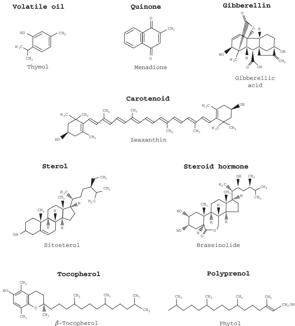
Figure 2.3 Chemical structure of selected terpenoids.
