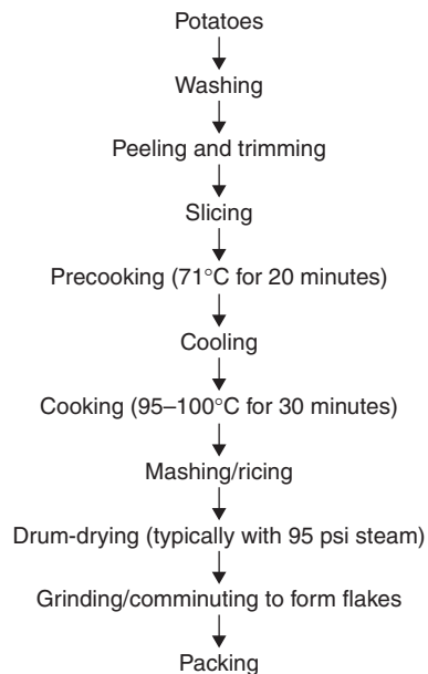
Figure 34.7 Process for making potato flakes.
