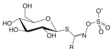
Figure 25.1 Structure of glucosinolate. Source: Rangavajhyala et al. 1998.
