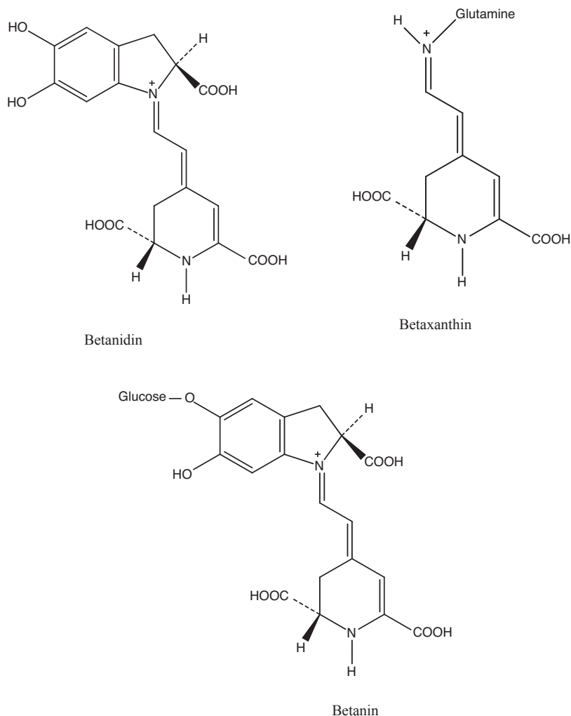
Figure 6.4 Structures of betalains in beet and Swiss chard.
