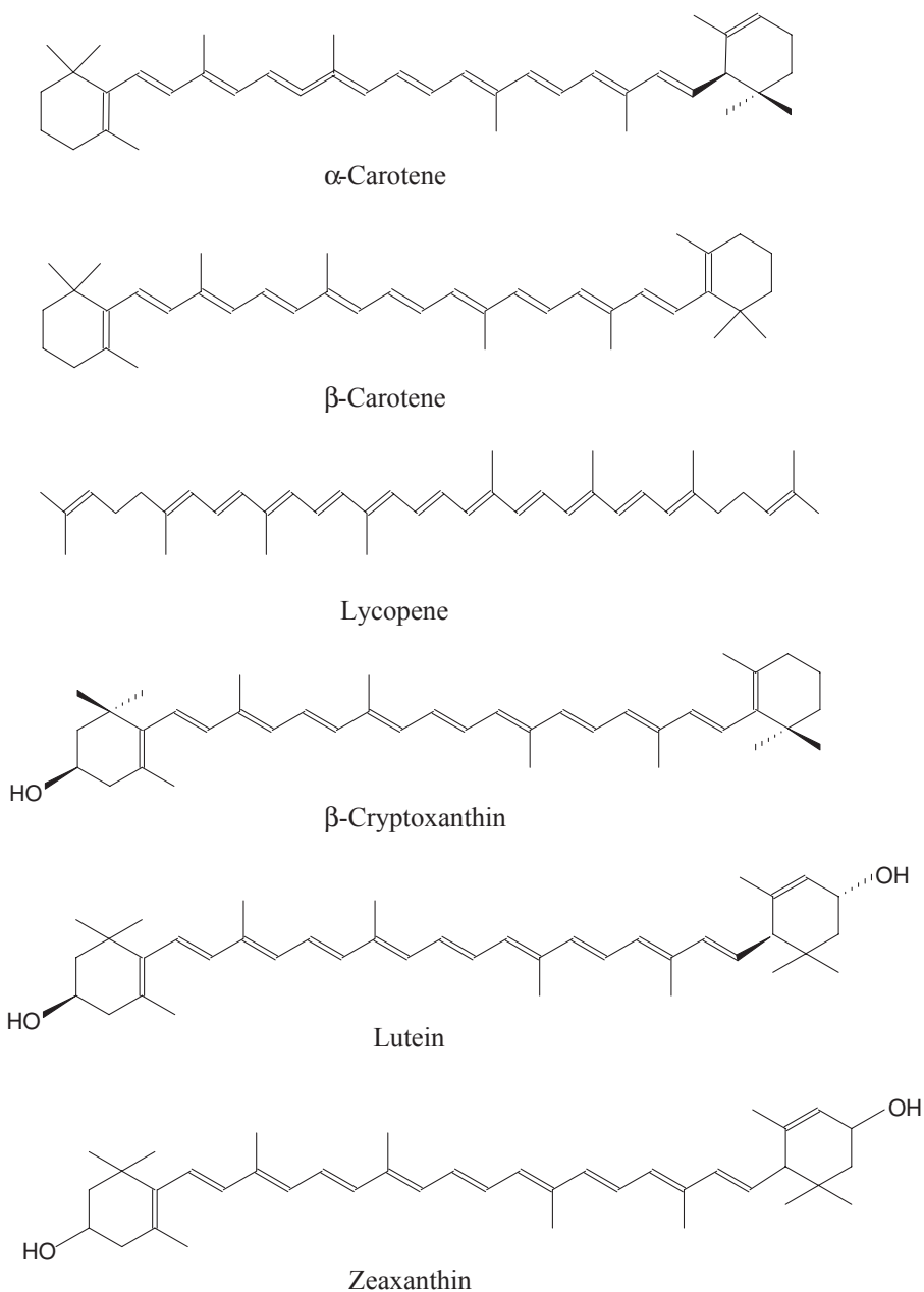
Figure 6.5 Chemical structures of \alpha - and \beta -carotene, lycopene, \beta -cryptoxanthin, lutein, and zeaxanthin.
