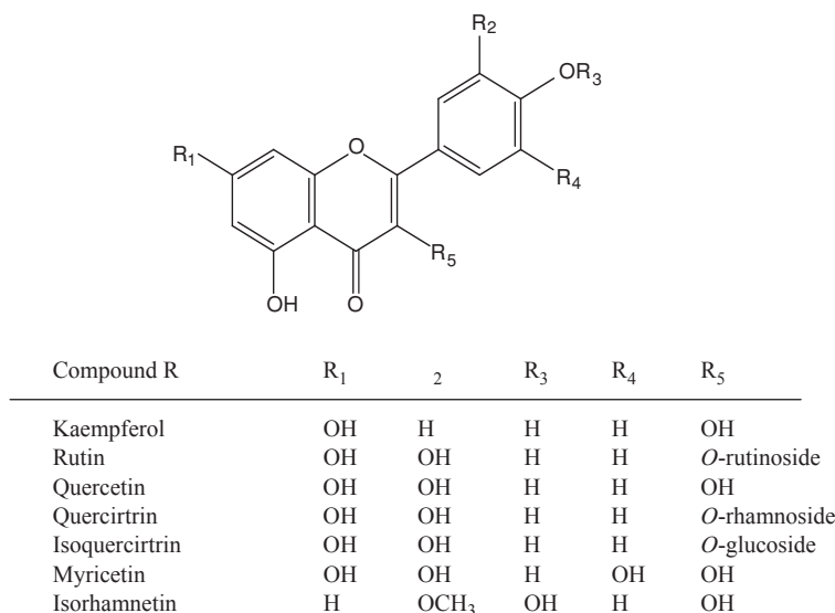
Figure 6.2 Structures of some flavonol derivatives.
