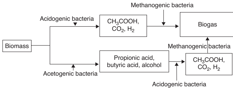
Figure 21.6 Anaerobic conversion of biogas.
