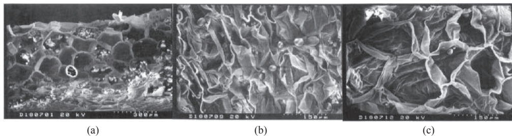
Figure 12.7 Scanning electron microscopy photograph of (a) untreated, (b) conventionally frozen (freezer, 0.1 MPa, -30^{\circ}\text{C} , 1 h), and (c) pressure-assisted frozen (400 MPa, 20 minutes) potato tissue. (From Koch et al. (1996).)
