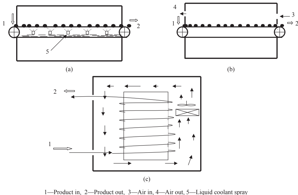
Figure 12.4 Belt freezers: (a) liquid spray, (b) air cooling, and (c) spiral belt.
