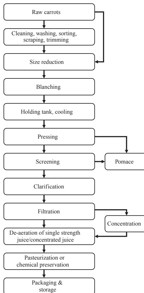
Figure 28.2 General flowchart for juice expression process.
