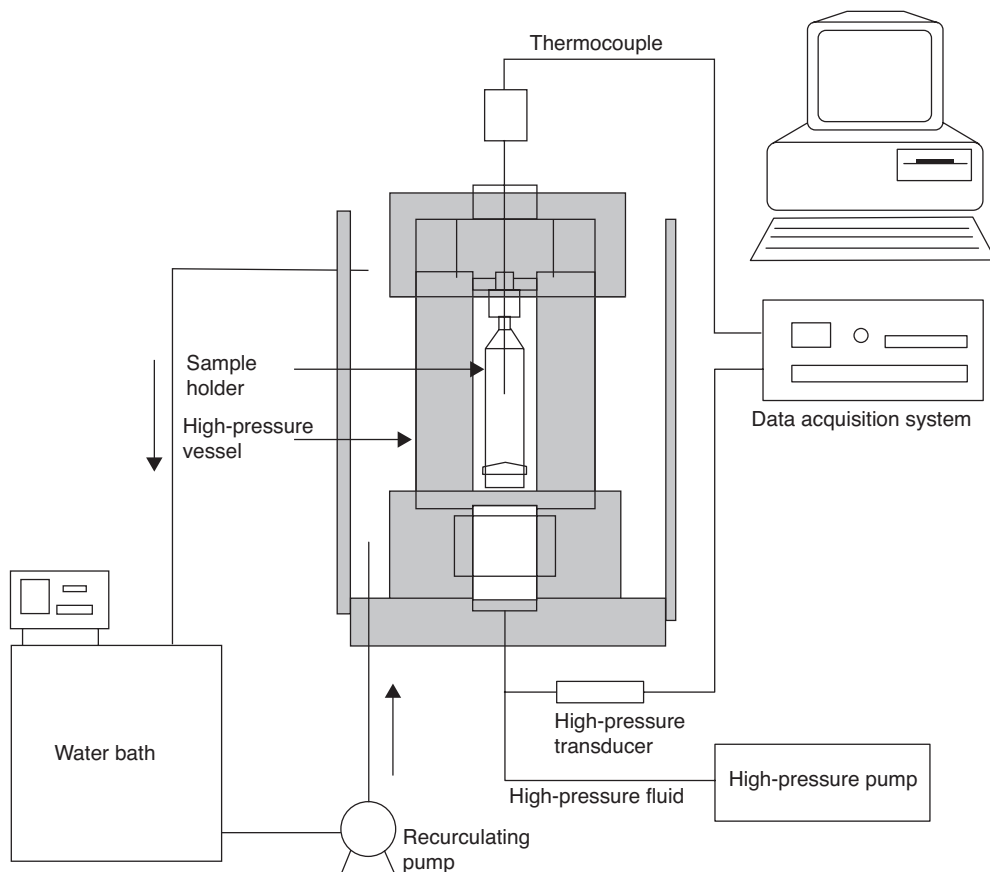
Figure 15.4 High-pressure processing of food. (Adapted from Patzca et al. (2007).)
