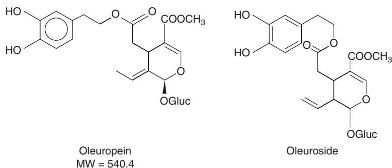
Figure 33.5 Structure of oleuropein and oleurosides.
