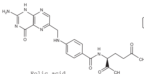
Folic acid
