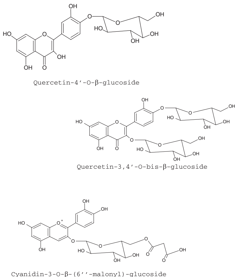
Figure 31.2 The main flavonoids in onion.
