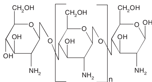
Figure 20.7 The structure of chitosan.
