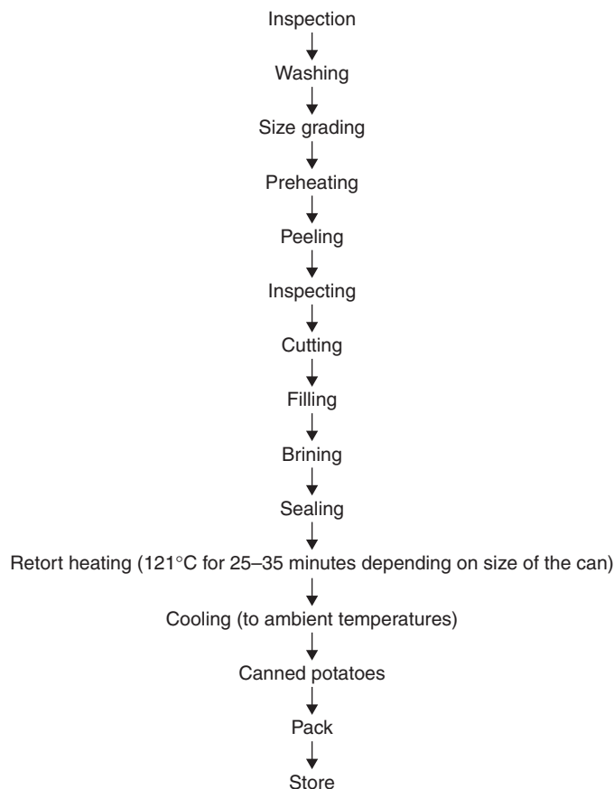
Figure 34.8 Process for canned potatoes.
