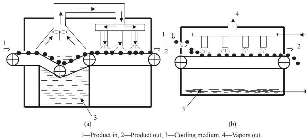
Figure 12.5 Cryogenic freezers: (a) immersion type, (b) spray type.
